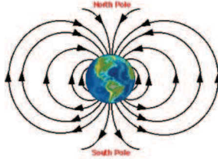
Figure 2. Sketch of the dipole field of the Earth. Note that every flux bundle emanating from the Earth's surface expands in width with height, reaching maximum width at its apex.
